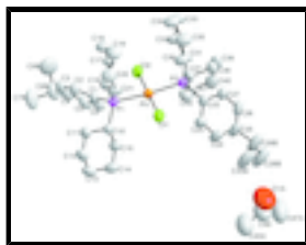
Fig. 1. A view of the title compound showing the numbering scheme of atoms and 50% probability displacement ellipsoids. Hydrogen atoms and the minor components of disordered parts are omitted for clarity.
